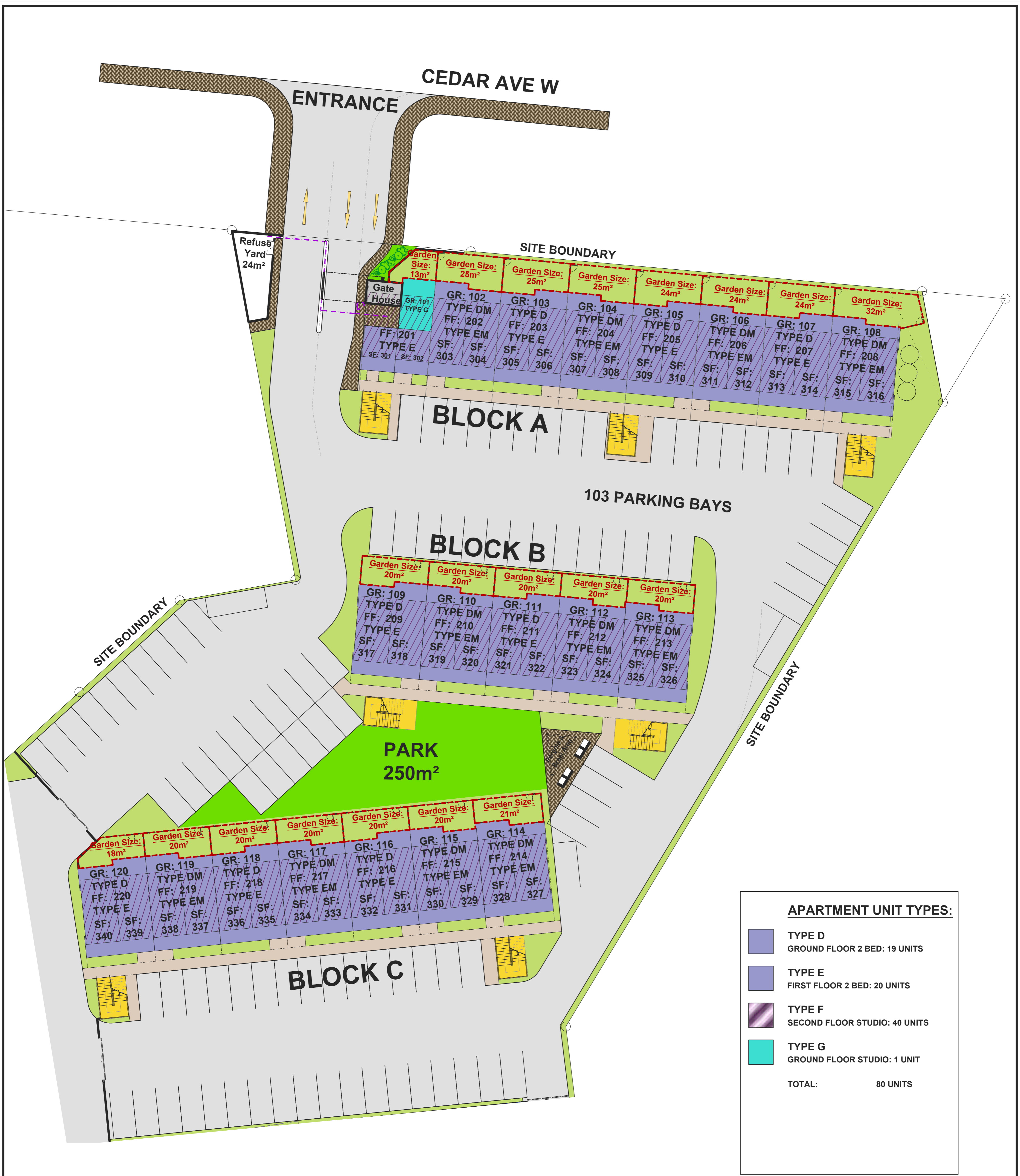
APARTMENT SITE PLAN SCALE 1 : 200 @ A1
